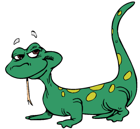
lizard lizard
