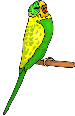
parakeet parakeet
