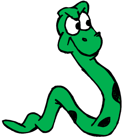
snake snake
